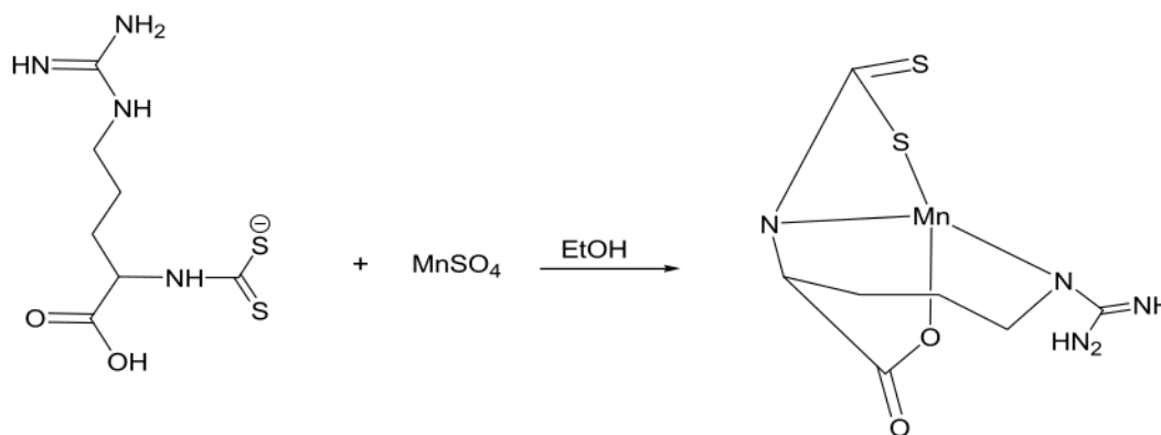
Fig. 1. Synthesis reaction of Mn (II) arginine dithiocarbamate.
