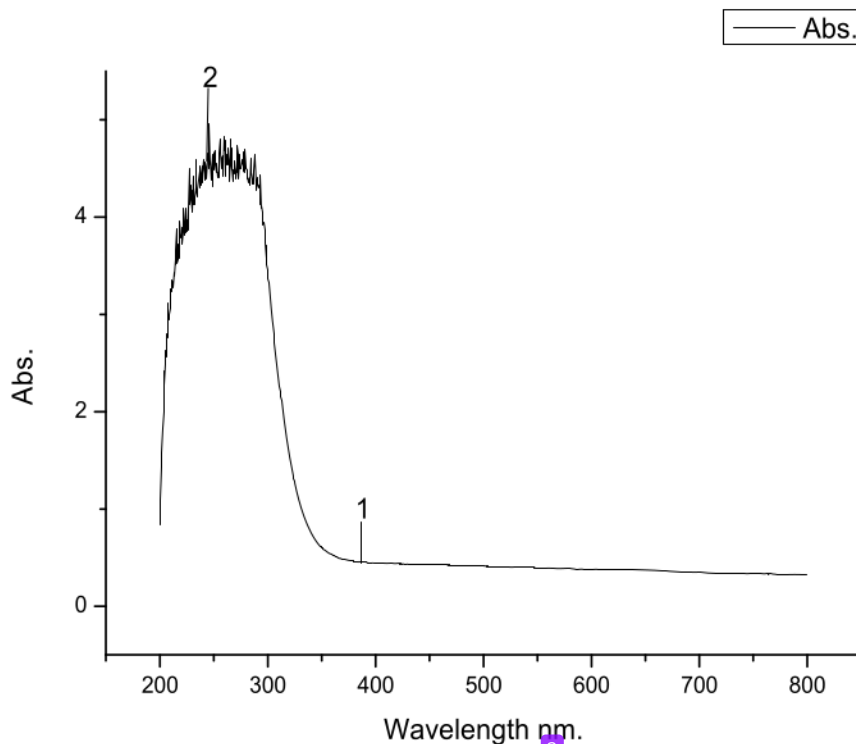
Fig. 2. UV-Vis Spectrum of Mn (II) arginine dithiocarbamate.
