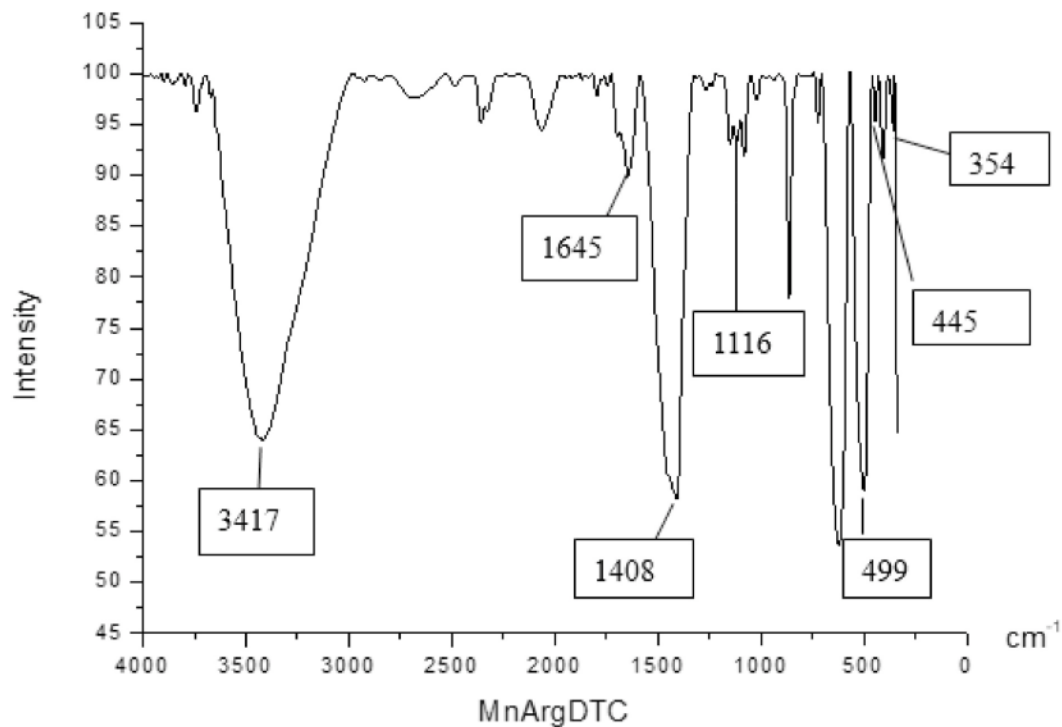
Fig. 3. IR Spectrum of Mn (II) arginine dithiocarbamate.
